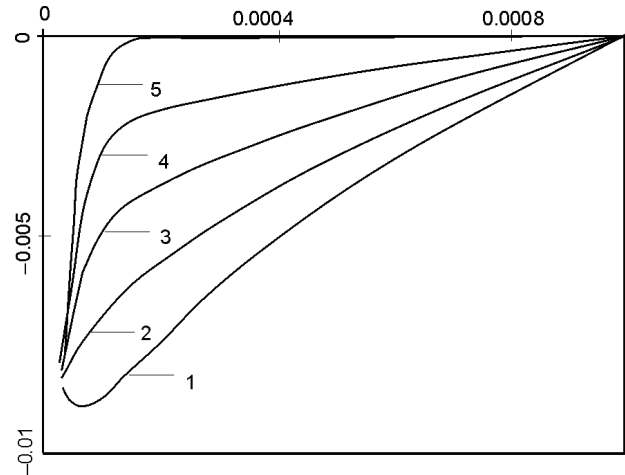
Fig. 2. Distributions of concentrating stresses in a layer for q = 2 \cdot 10^1 , d = 5 \cdot 10^{-3} , \tau^* = 1,5 \cdot 10^{-2} ; curve 1 for \eta = 1 , 2 - \eta = 0,75 , 3 - \eta = 0,5 , 4 - \eta = 0,25 , 5 - \eta = 0
