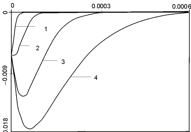
Fig. 4. Behaviour of concentrating stress distributions in time for \eta=1 , q = 2 \cdot 10^2 , d = 5 \cdot 10^{-1} ; curve 1 for \tau^* = 5 \cdot 10^{-4} , 2 - \tau^* = 5 \cdot 10^{-3} , 3 - \tau^* = 5 \cdot 10^{-2} , 4 - \tau^* = 5 \cdot 10^{-1}
