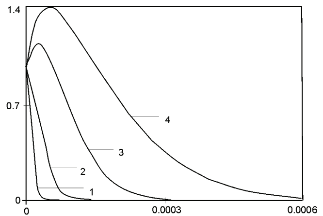
Fig. 3. Behaviour of total admixture concentration distributions in time for \eta = 1 , q = 2 \cdot 10^2 , d = 5 \cdot 10^{-1} ; curve 1 for \tau^* = 5 \cdot 10^{-4} , 2 - \tau^* = 5 \cdot 10^{-3} , 3 - \tau^* = 5 \cdot 10^{-2} , 4 - \tau^* = 5 \cdot 10^{-1}
