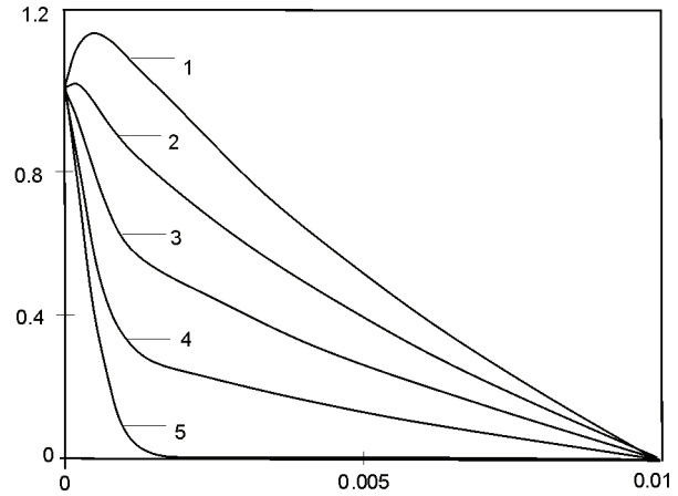
Fig. 1. Distributions of total admixture concentration in a layer for q = 2 \cdot 10^1 , d = 5 \cdot 10^{-3} , \tau^* = 1,5 \cdot 10^{-2} ; curve 1 for \eta = 1 , 2 - \eta = 0,75 , 3 - \eta = 0,5 , 4 - \eta = 0,25 , 5 - \eta = 0
