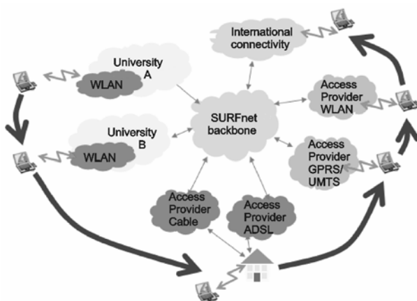
Fig. 1. Roaming users
